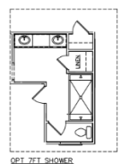
OPT. SECOND FLOOR PLAN (SCALE: 1/8"=1'-0")
