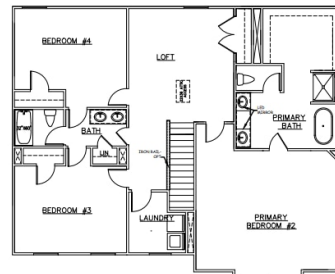
OPT. SECOND FLOOR PLAN
