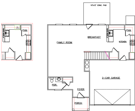
FIRST FLOOR PLAN (SCALE 1/8"=1'-0")
