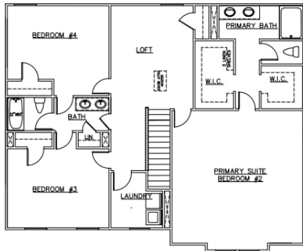
SECOND FLOOR PLAN (SCALE 1/8"=1'-0")
