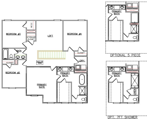
OPT. SECOND FLOOR PLAN
