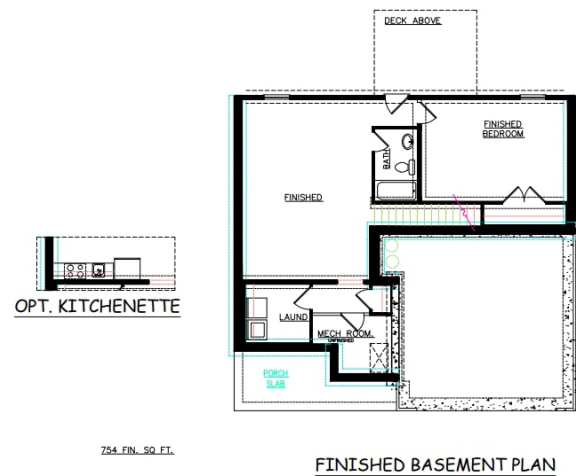
FINISHED BASEMENT PLAN
