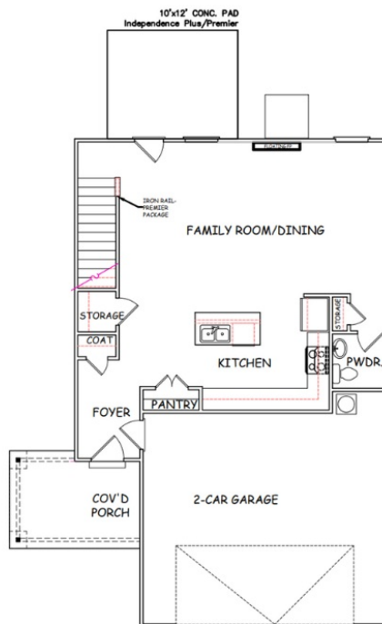
FIRST FLOOR FARMHOUSE
