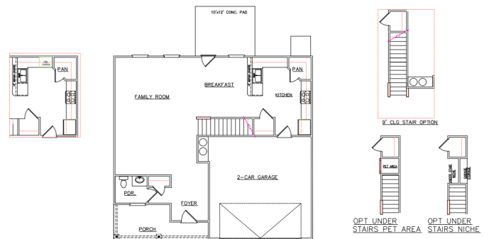
FIRST FLOOR PLAN (SCALE 1/8"=1'-0")
