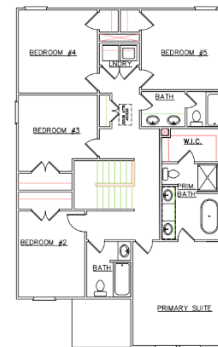
SECOND FLOOR PLAN S046 1/16" = 1'
