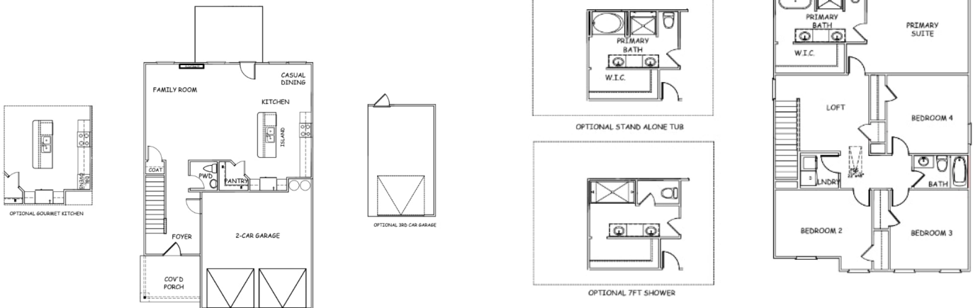
OPT SECOND FLOOR PLAN (SCALE 1/8" = 1')
