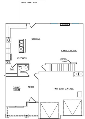
FIRST FLOOR PLAN (SCALE 1/8"=1'-0")
