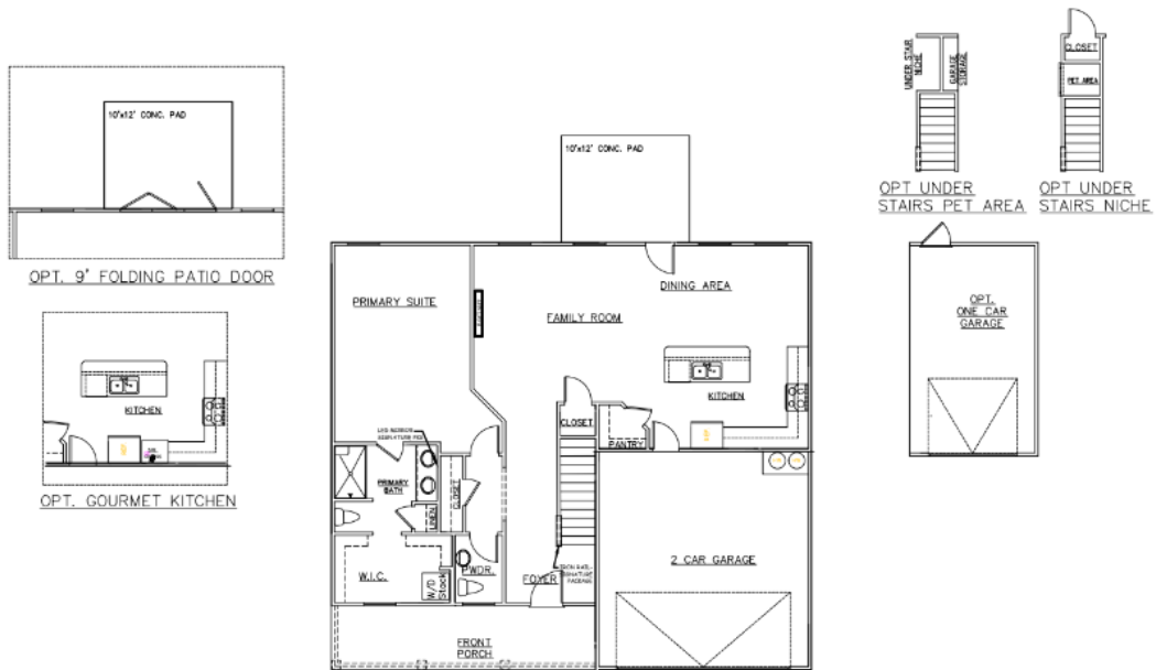
FIRST FLOOR PLAN (SCALE 1/8"=1'-0")
