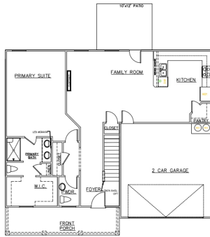
FIRST FLOOR PLAN (SCALE 1/8"=1'-0")
