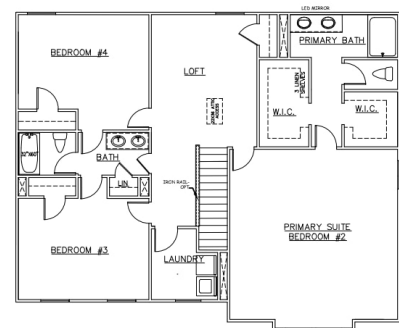
SECOND FLOOR PLAN (SCALE 1/8"=1'-0")
