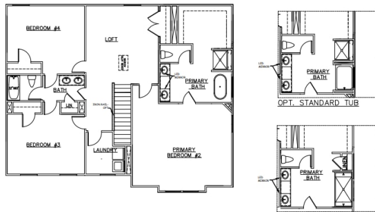
OPT. SECOND FLOOR PLAN
