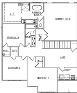
SECOND FLOOR PLAN (SCALE 1/8"=1'-0")
