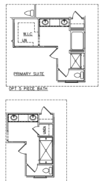
OPT. SECOND FLOOR PLAN
