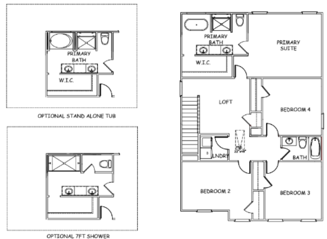
OPT SECOND FLOOR PLAN (SCALE 1/8"=1'-0")
