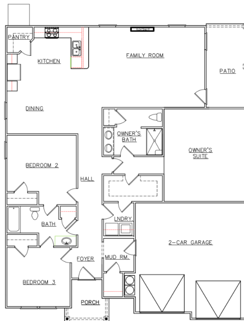
1ST FLOOR
