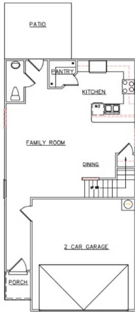
FIRST FLOOR PLAN-NELSON
