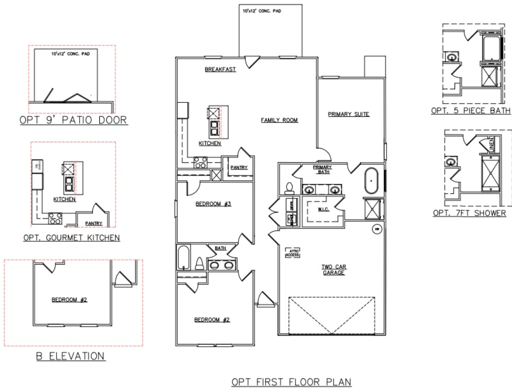
1ST FLOOR
