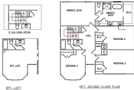
OPT. SECOND FLOOR PLAN
