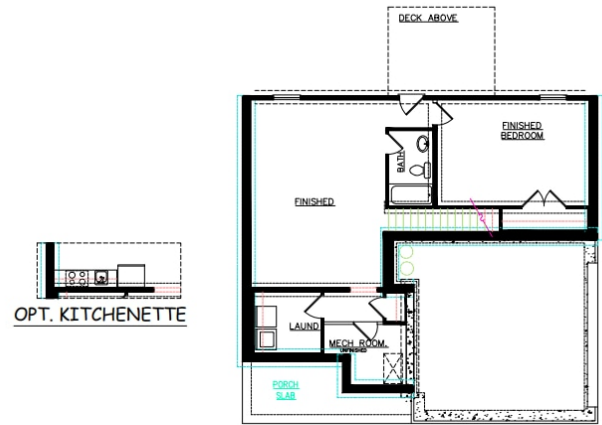
FINISHED BASEMENT PLAN
