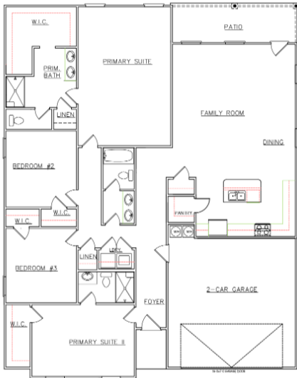
FIRST FLOOR PLAN (SCALE: 1/8" = 1')
