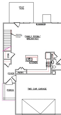
1ST FLOOR
