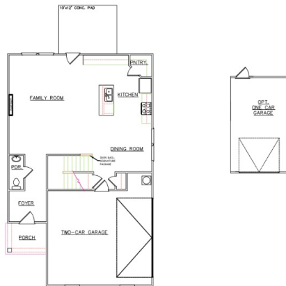
FIRST FLOOR PLAN (SCALE 1/8"=1'-0")
